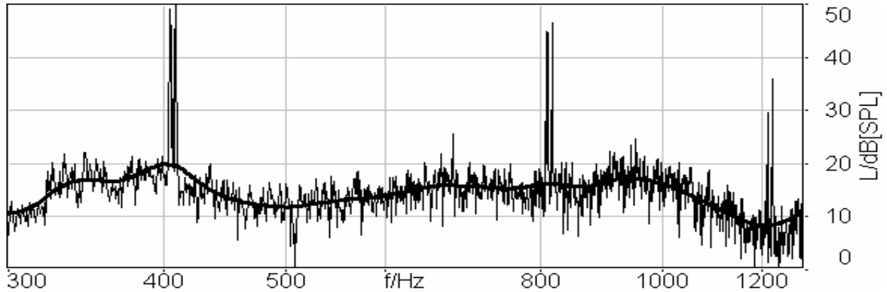
Fig. 1: DFT spectrum with several double tones and smoothed spectrum (bold line).
