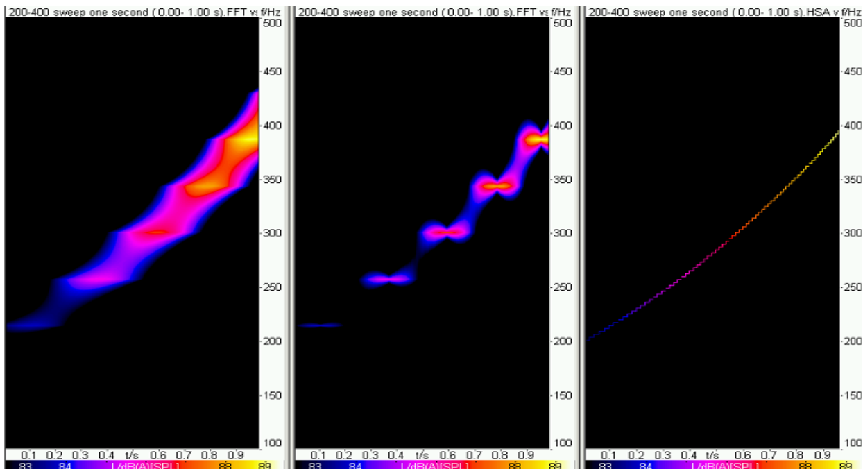
Fig. 4: High-resolution Spectral Analysis [6], A-weighted spectra vs. time: left, Hanning-windowed FFT vs. time (left), middle, no window; right, High-Resolution Spectral Analysis (HSA): window deconvolved and frequency resolution multiplied 16X.
