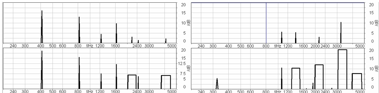
Fig. 3: Comparison of the TNR (upper) automated procedure and automatic DIN 45681 results (lower), for a fan noise (left) and a defective automobile tire (right). A comparison of the methods may be found in the Appendix.
