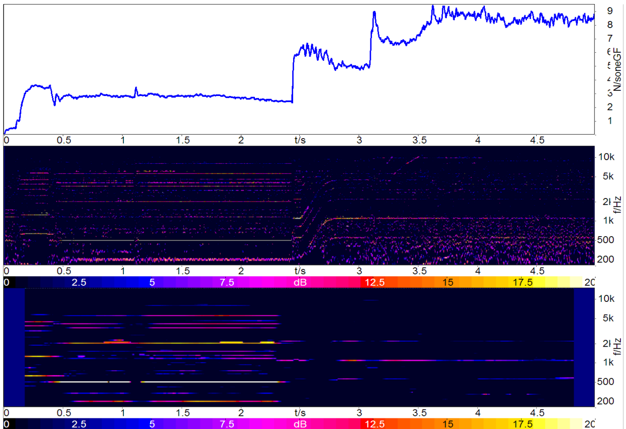
Fig. 9: Printer including rapid frequency-sweep. Upper, loudness vs. time (DIN 45631/A1 [7]); Tone-to-Noise Ratio vs. time: middle, by HSA (4x frequency resolution multiplication), block size 4096 points; \Delta t = 92.9 ms, \Delta f = 2.69 Hz; lower, calculated conventionally (16384 Hanning, \Delta t = 371.5 ms, \Delta f = 2.69 Hz).
