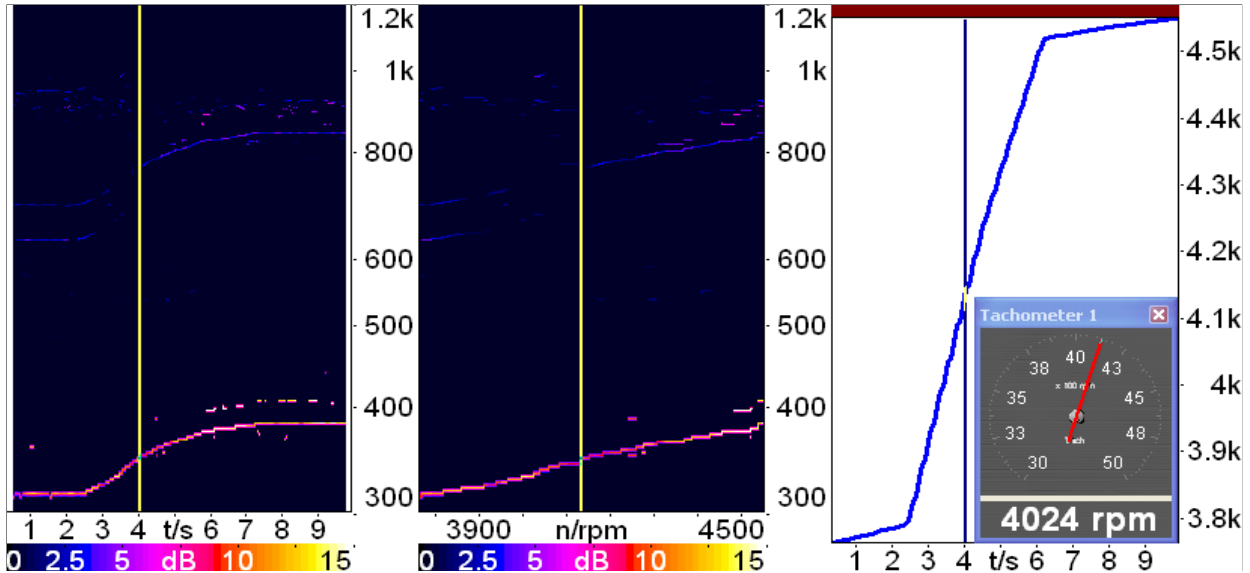
Fig. 10: Computer cooling fan, Prominence Ratio spectrum by conventional DFT method (16384 points, Hanning): left, vs. time, center, vs. RPM; right: the RPM vs. time. It may be useful to determine prominent-tone spectra and magnitudes versus other references than time, for example RPM, air pressure, flow rate, stepping rate, temperature, voltage, etc.
