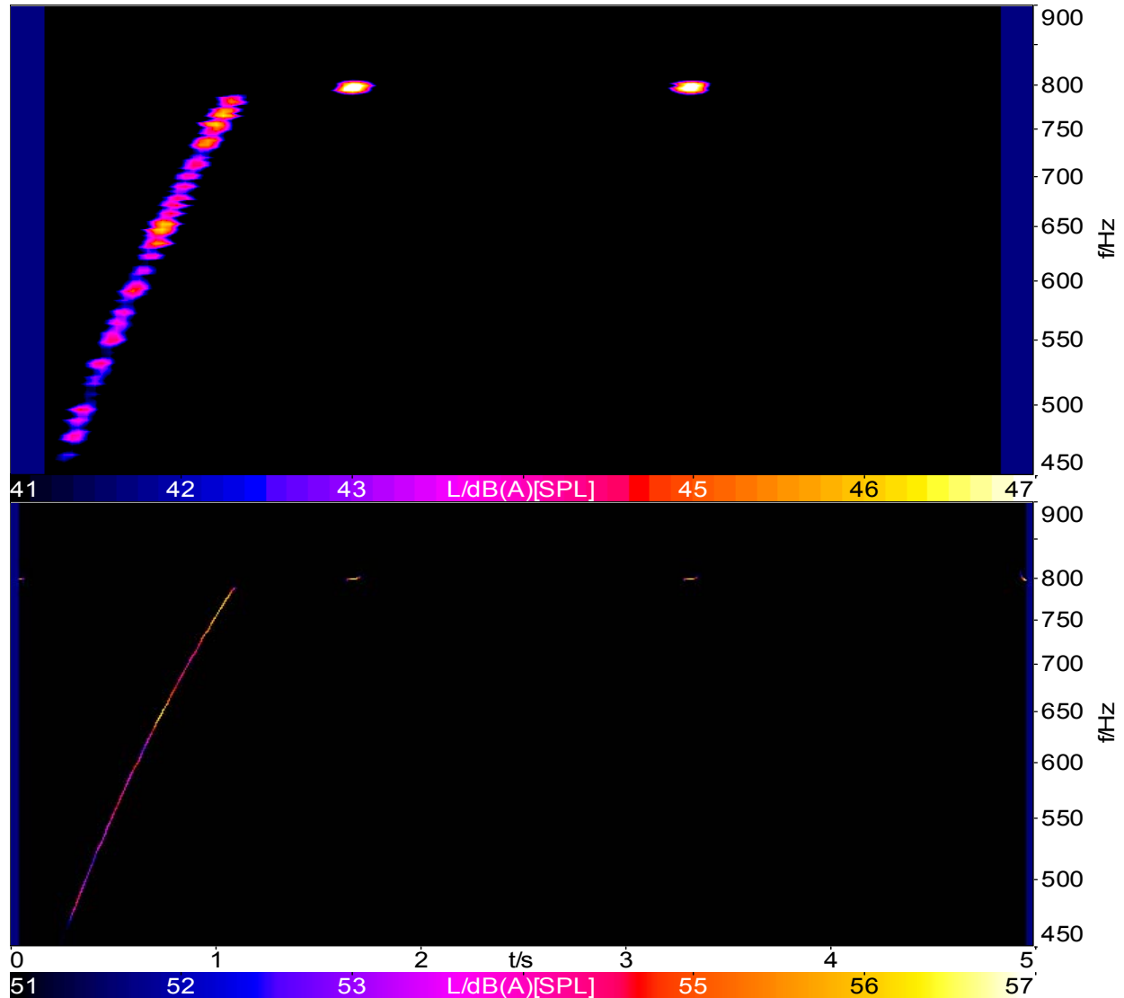
Fig. 5: A-weighted spectra vs. time of a situation with three time-varying subjectively prominent tones; a sweep tone 500-800 Hz at constant 57 dB[SPL] followed by two 800 Hz, 57 dB[SPL] tones of 70 ms duration each, all in continuous random pink noise of 60 db[SPL]. Upper: FFT vs. time 16384 points, 96% overlap, Hanning window. Lower: High-resolution Spectral Analysis (HSA) vs. time, 4096-point FFT, 99% overlap: \Delta f = 0.673 Hz, \Delta t = 92.9 ms. Note: the level scales differ by 10 dB. In the upper illustration the momentary tones occupy less than 1/5 the duration of a 16384-point Fourier block at this sampling rate and therefore are not represented at actual level, although they indicate higher than any point along the sweeping tone.
